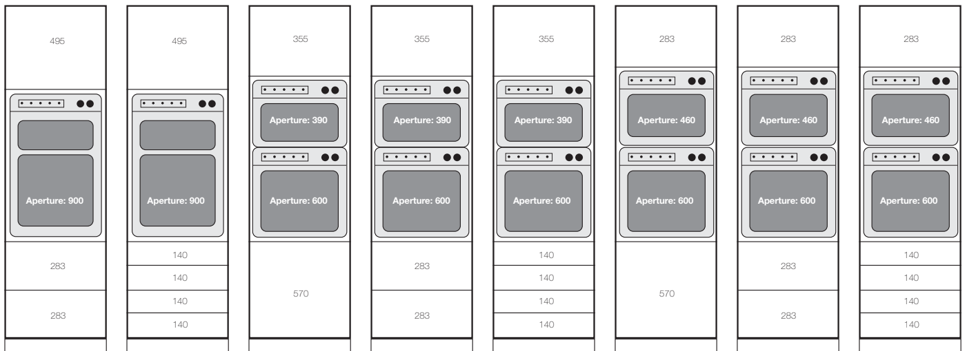
Tall Appliance Housing 900mm Aperture Type D2
